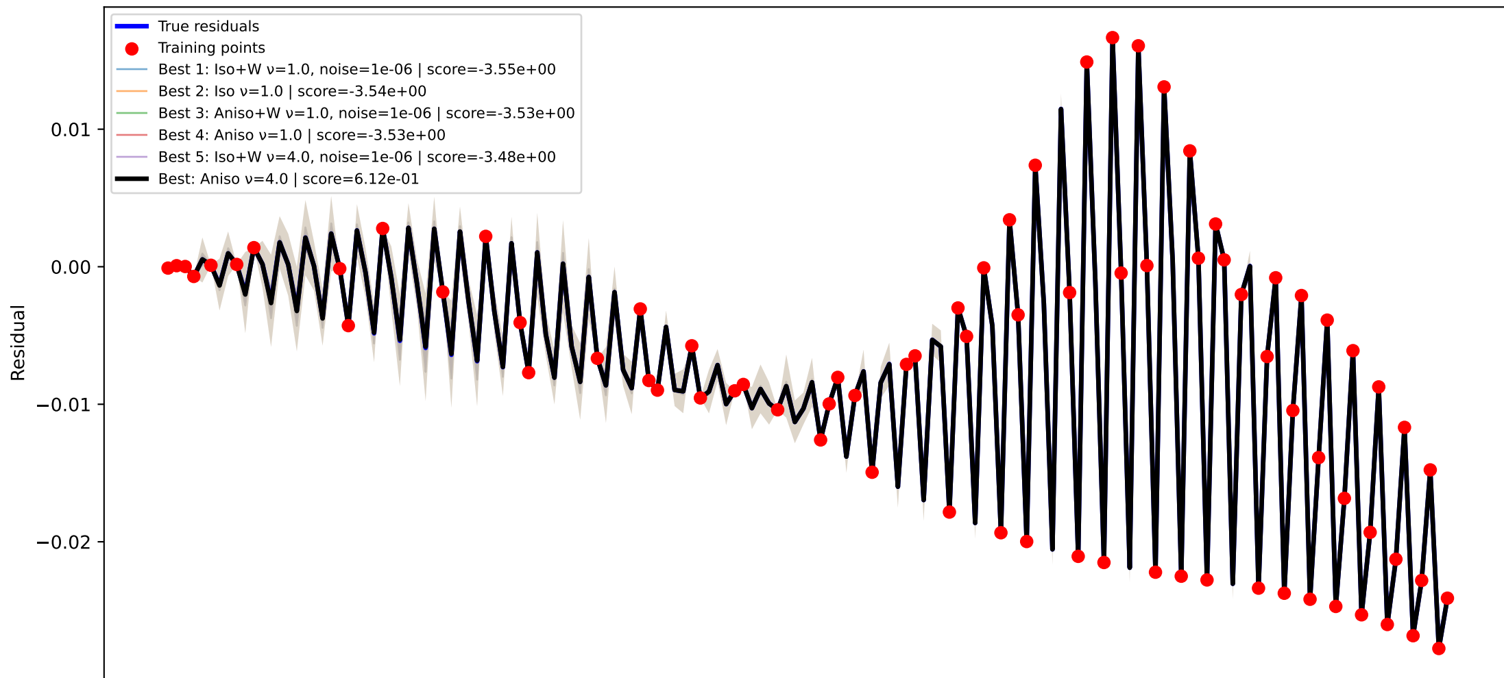
GPR kernel comparison node=50 RMSE=2.101e-05, train RMSE=7.440e-10
